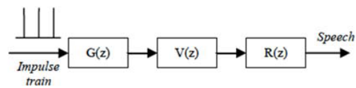
Figure 1: Generalized speech production model (Iliev, 2012).
